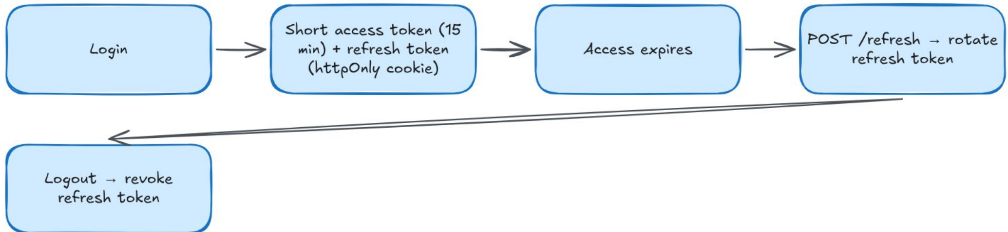
Access + refresh token pattern
